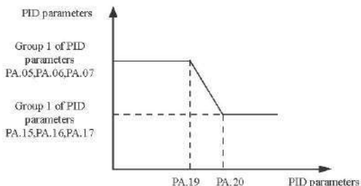
Figure 4-24 PID parameters switchover
