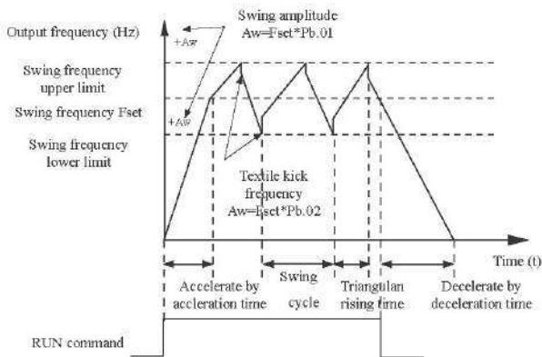
Figure 4-26 Swing frequency control
